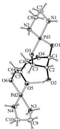
Figure 4. The structure of [(en)_2Pd_2(\beta\text{-D-Galf1,3,5,6H}_4)] molecules in crystals of 4 (50% probability ellipsoids). The intramolecular O2\text{-H}\cdots O5 bond is shown as a gray bar. Distances [Å] and angles [°]: from Pd1 to: O1 2.010(2), O3 2.014(2), N2 2.040(3), N1 2.044(3); from Pd2 to: O6 1.992(2), O5 2.016(2), N4 2.026(3), N3 2.054(3); O1–C1 1.383(4), O2–C2 1.439(4), O3–C3 1.408(4), O4–C1 1.441(4), O4–C4 1.447(4), O5–C5 1.431(4), O6–C6 1.423(4), C1–C2 1.521(5), C2–C3 1.528(5), C3–C4 1.556(4), C4–C5 1.524(4), C5–C6 1.525(4); galactose bond angles with largest deviation from the tetrahedral angle: C1–C2–C3 101.6(3), C2–C3–C4 101.7(3); torsion angles: O1–C1–C2–O2 -160.0(3) , O2–C2–C3–O3 160.0(3), O3–C3–C4–O4 98.0(3), O4–C4–C5–O5 71.0(4), O5–C5–C6–O6 49.6(4); intramolecular hydrogen bond: O2\text{-H}\cdots O5 1.64(4), O2\cdots O5 2.544(3) Å, O2\text{-H}\cdots O5 172(4)°; puckering parameters [13] of the furanose ring O4–C1...: Q_2 = 0.407(3) Å, \phi_2 = 248.5(5)^\circ , the conformation therefore being close to E_{C_2} (ideal \phi_2: 252^\circ ).
