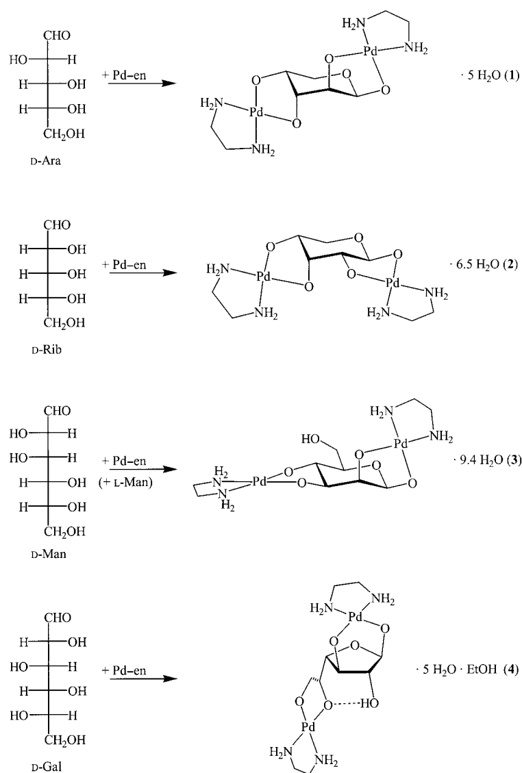
Scheme 2. Reaction scheme for the four crystalline compounds 1–4.
