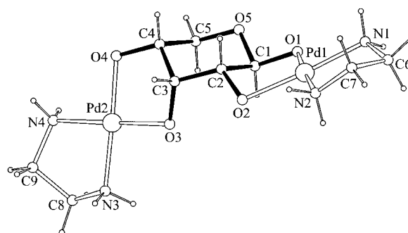
Figure 2. The structure of the dimetalated ribose complex [(\text{en})_2\text{Pd}_2(\beta\text{-D-Ribp1,2,3,4H}_4)] in a preliminary structure analysis of 2 . Mean distances [ \text{\AA} ]: Pd–O 2.009, Pd–N 2.029; add the digit "2" to each atomic label in the Figure to obtain the label in the crystallographic information file (CIF).
